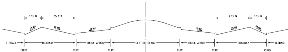
CIRCULATORY ROADWAY AND TRUCK APRON CROSS SECTION
