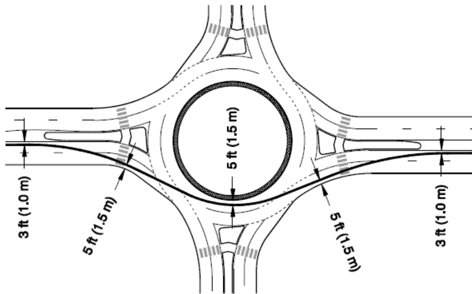
OFFSETS AND FASTEST THROUGH PATH FOR A MULTI-LANE ROUNDABOUT
