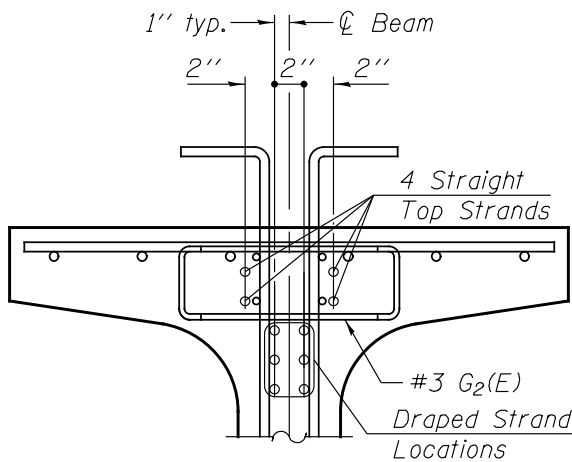
IL36 THRU 72 BEAM SECTION
