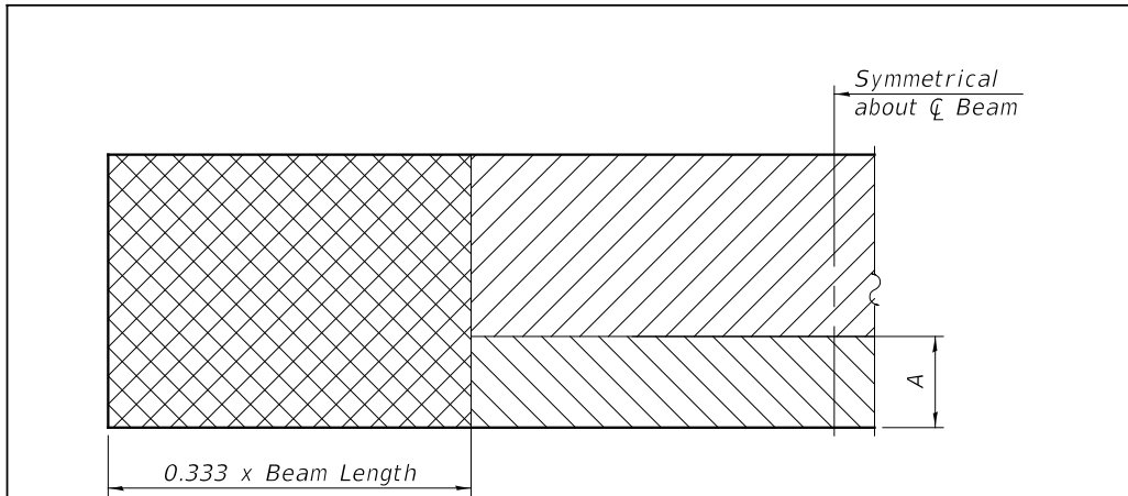
ELEVATION OF PRESTRESSED BEAM PATCH REPAIR AREAS
