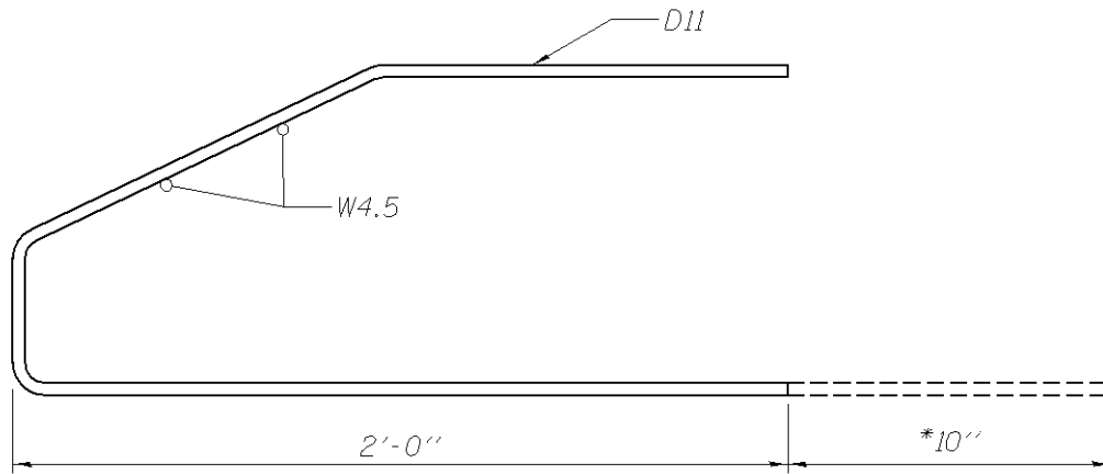
IL36 THRU 72 BEAMS (M 2 thru M 4 WWR)
