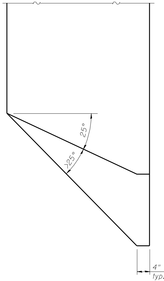
PLAN VIEW SHOWING END OF TYPICAL DECK BEAM
