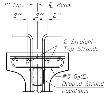
IL27 BEAM SECTION
