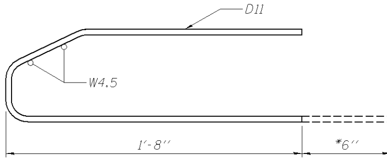
IL27 BEAM (M 2 and M 3 WWR)
