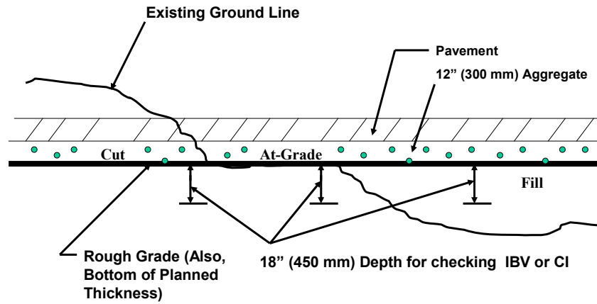
Case 1. Improved Subgrade - Aggregate
