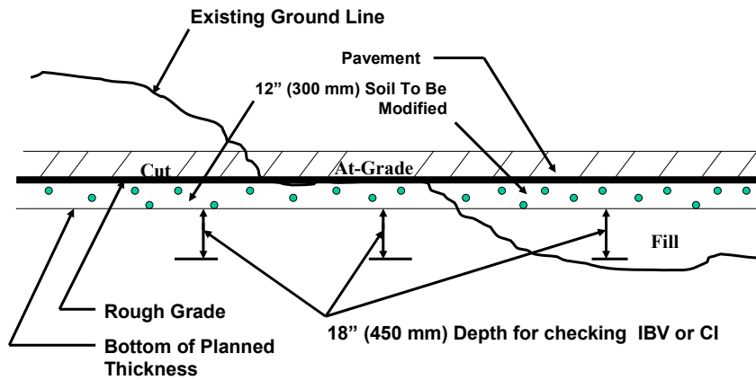
Case 2. Improved Subgrade – Modified Soil
