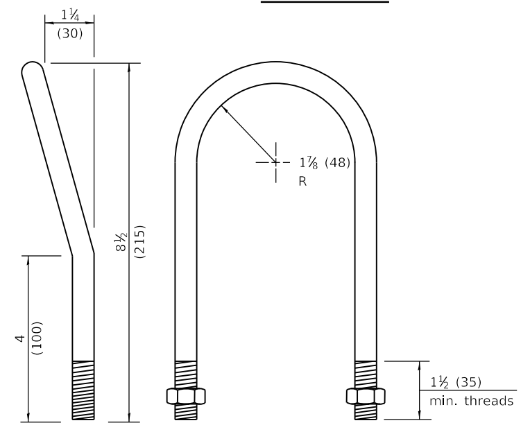
SECTION C-C
