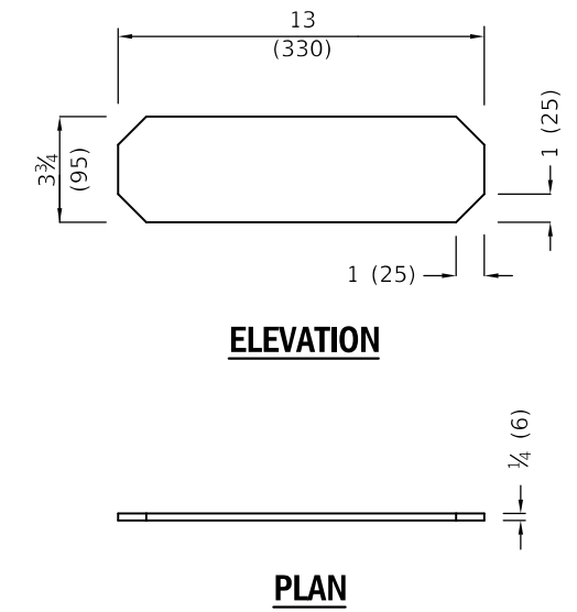
ANGLE CUT TUBE ASSEMBLY - END PLATE
