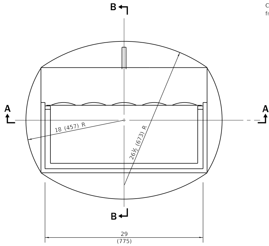
CAST FRAME
