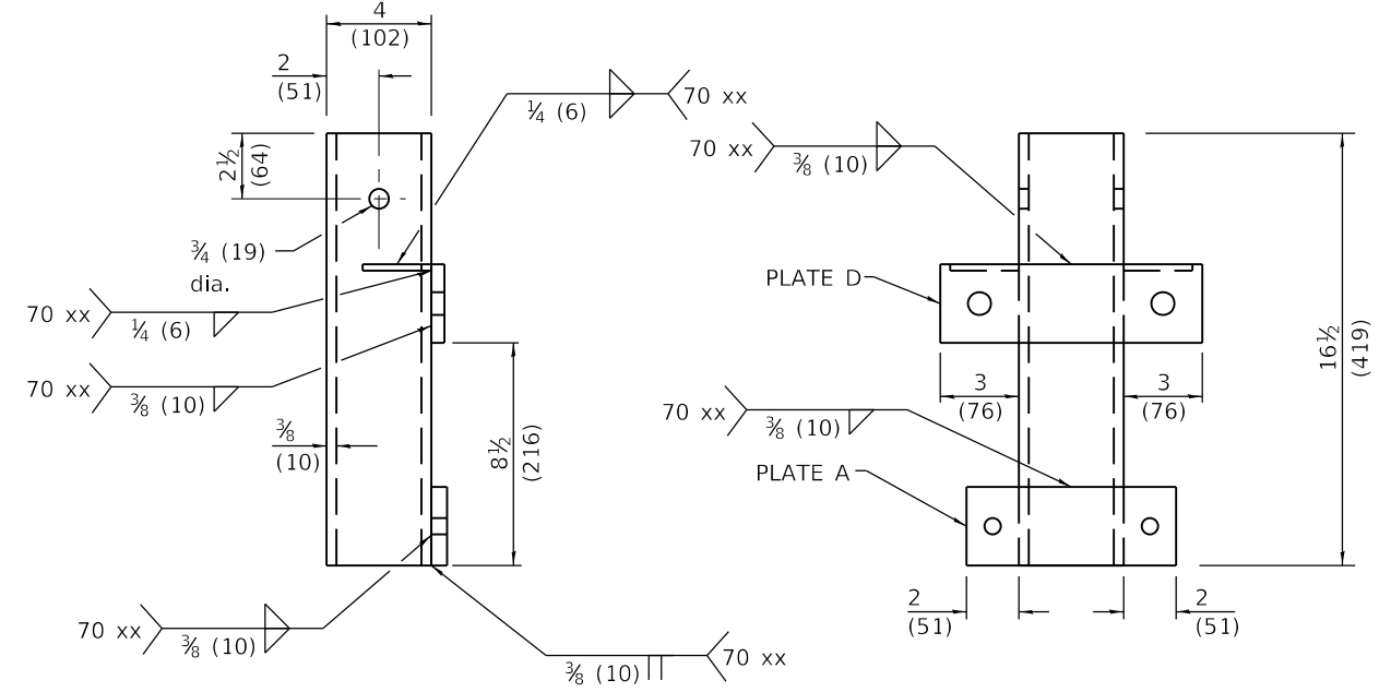
SIDE VIEW
