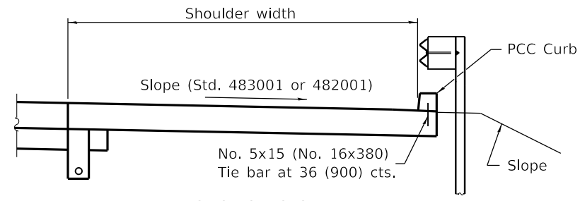
SECTION C-C
