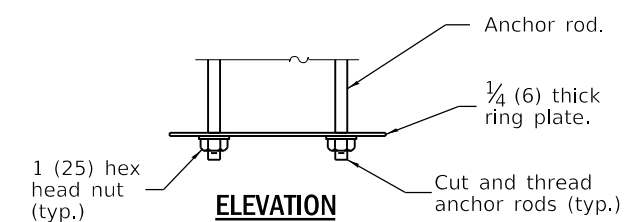
RING PLATE DETAIL ELEVATION
