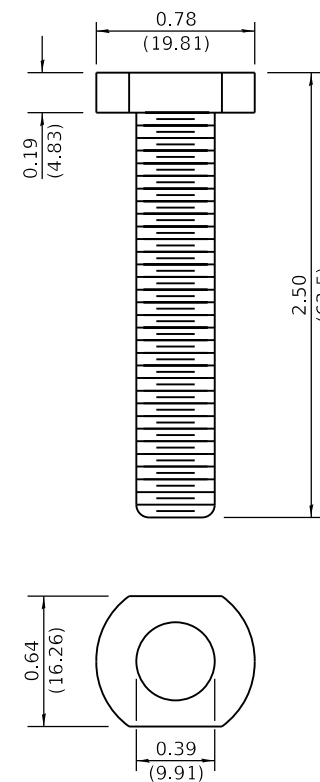
ALUMINUM CLIP NUT, BOLT AND WASHER ASSEMBLY
