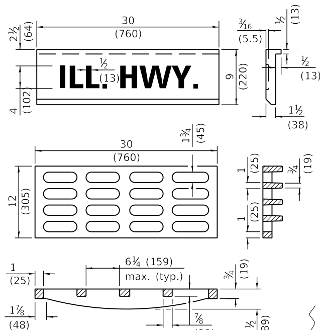
GRATE AND COVER TYPE 2B
