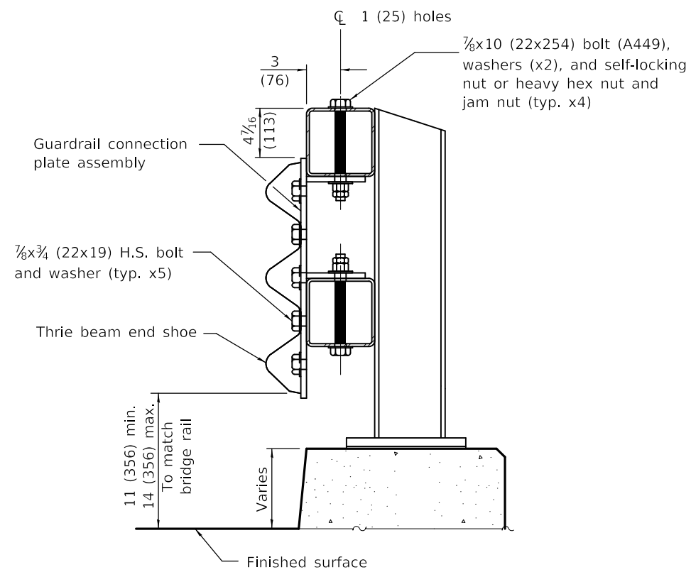
SECTION C-C
