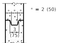
DETAIL of OPTIONAL JOINT
