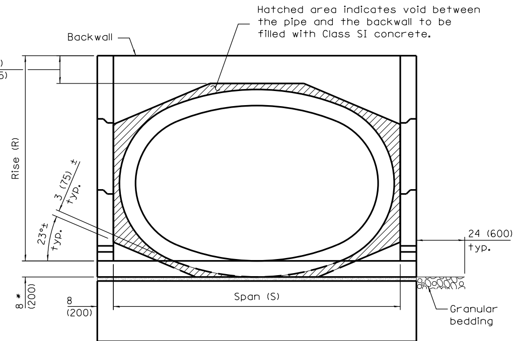
END VIEW
