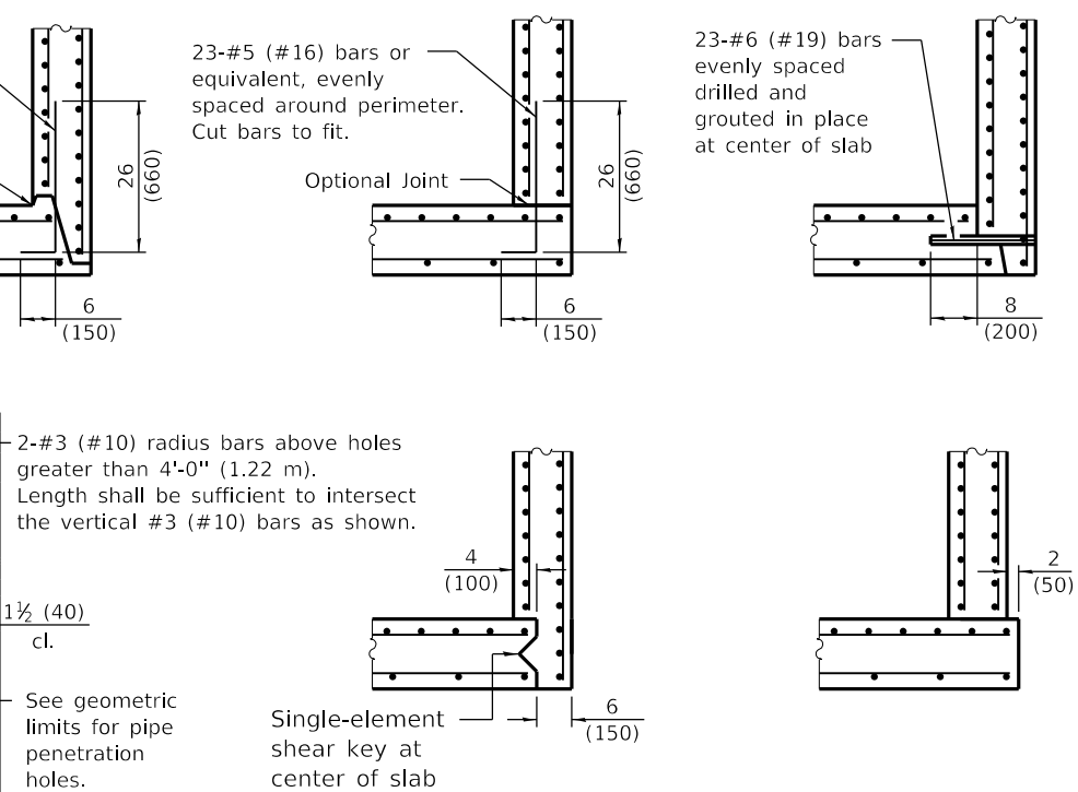
BASE SLAB JOINT CONFIGURATIONS
