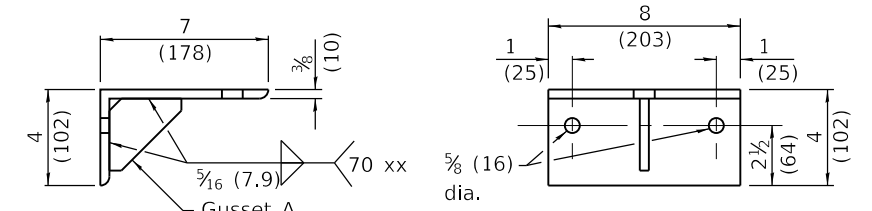
BRACKET B
