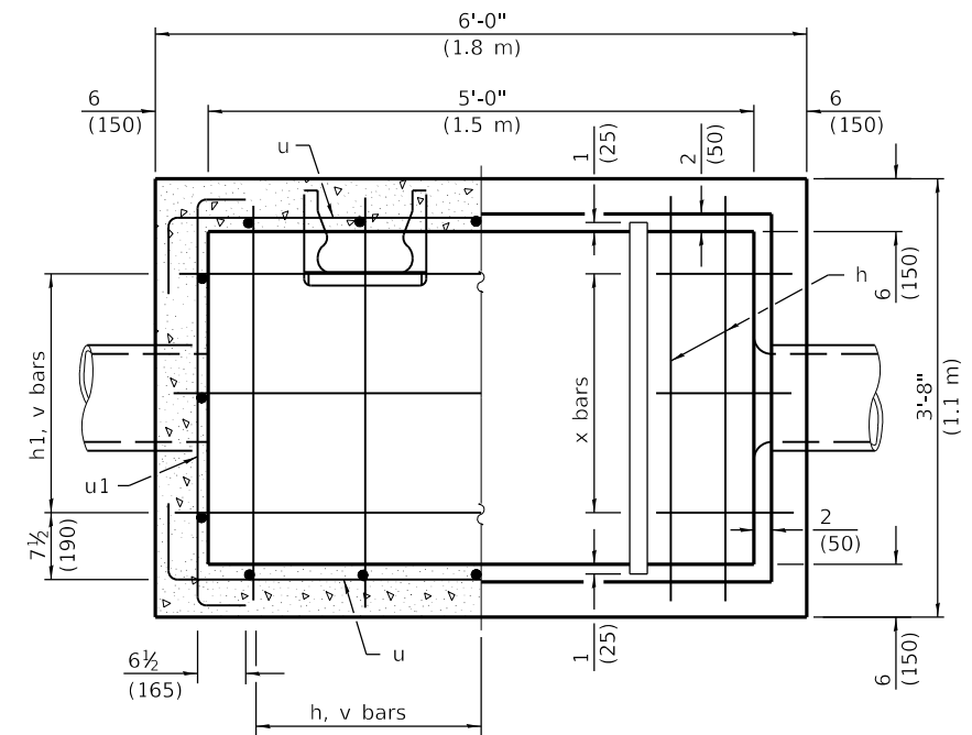
SECTION A-A (Grating removed to show plan of baffles.)
