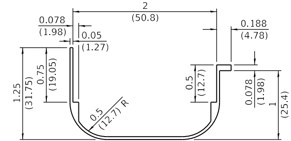
SIGN MOLDING
