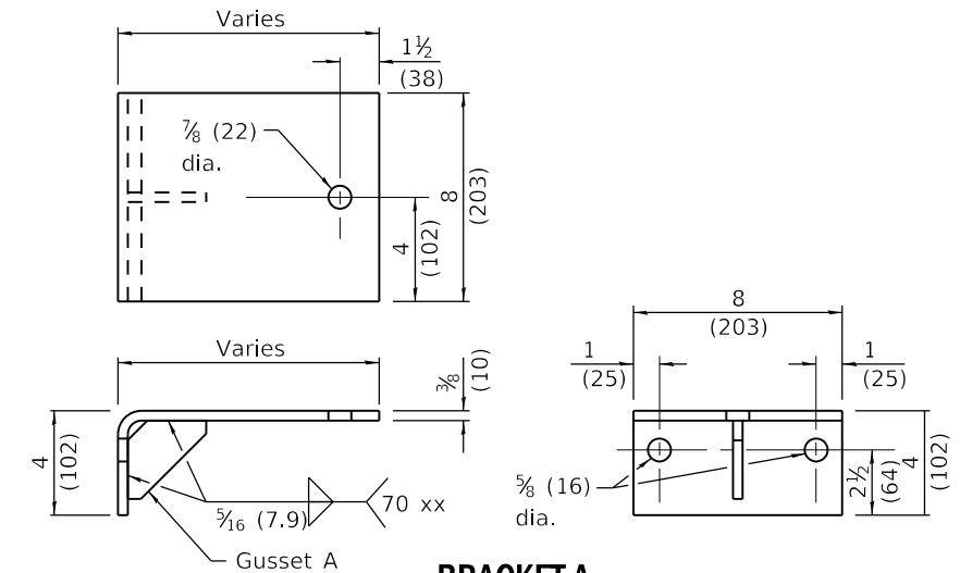
BRACKET A
