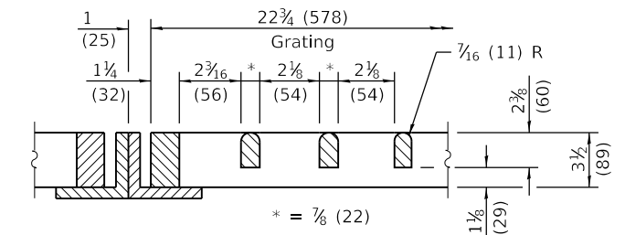
DETAIL B
