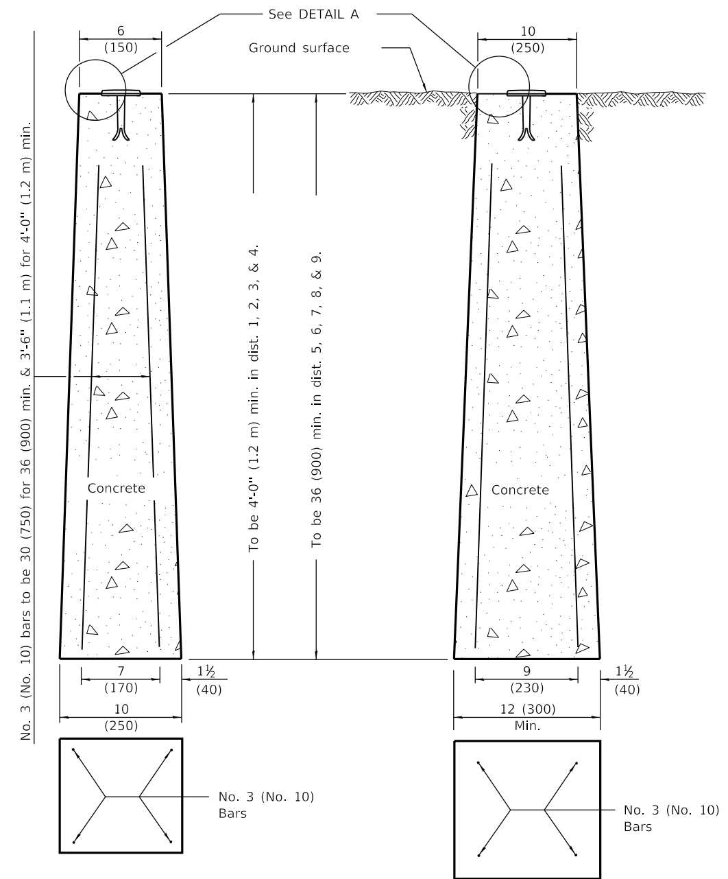
PRECAST MARKER
