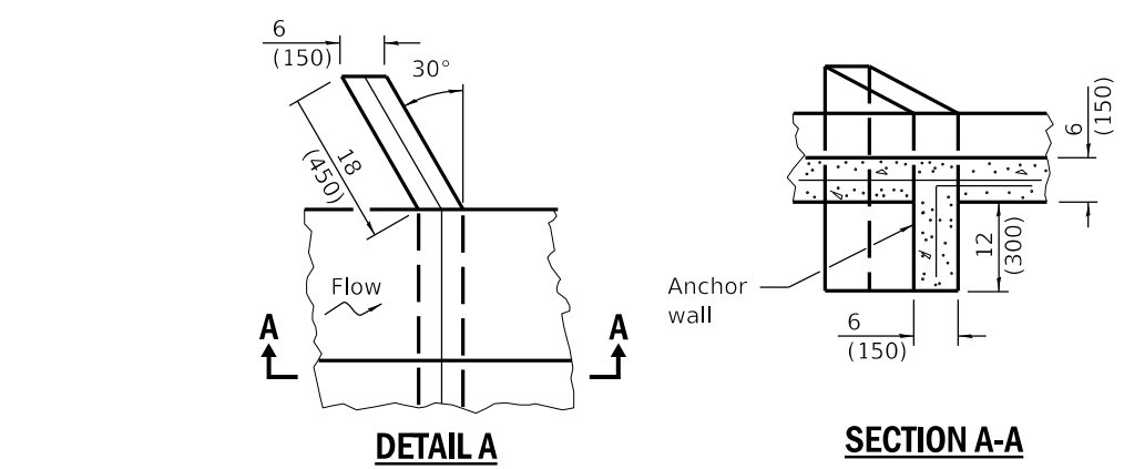
DETAIL OF ANCHOR WALL
