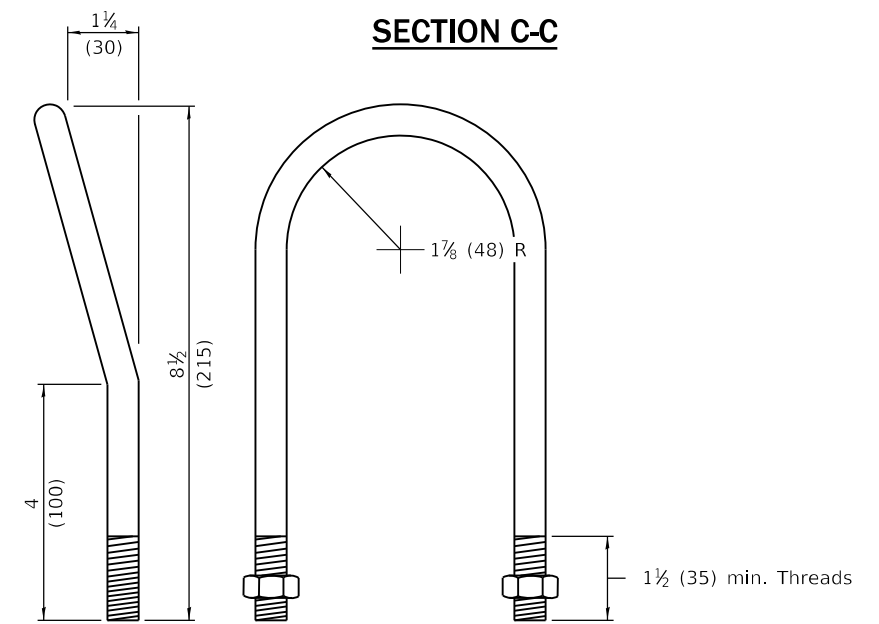
1/2 (M12) U BOLT (2-required)
