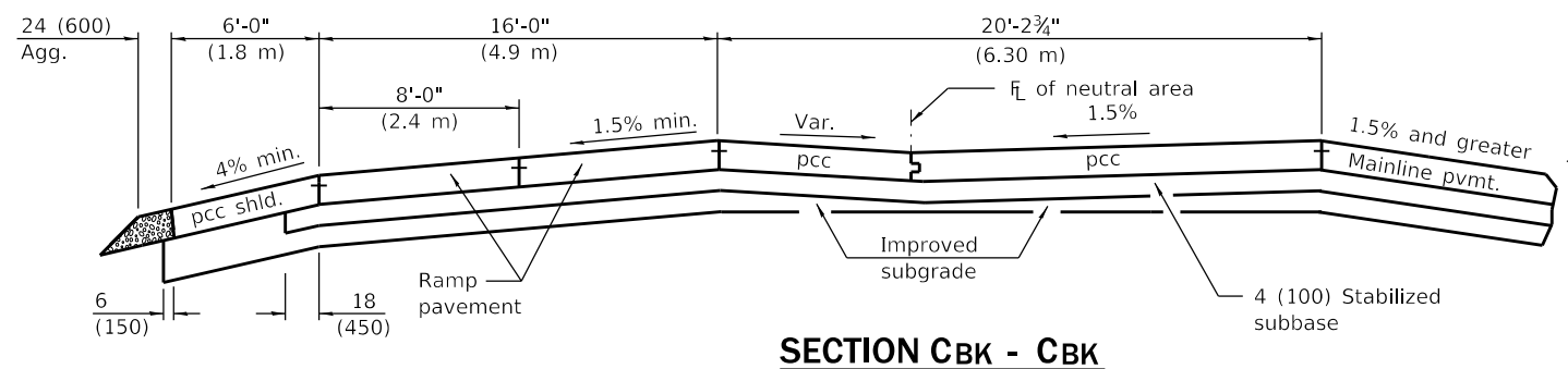
SECTION CAH - CAH
