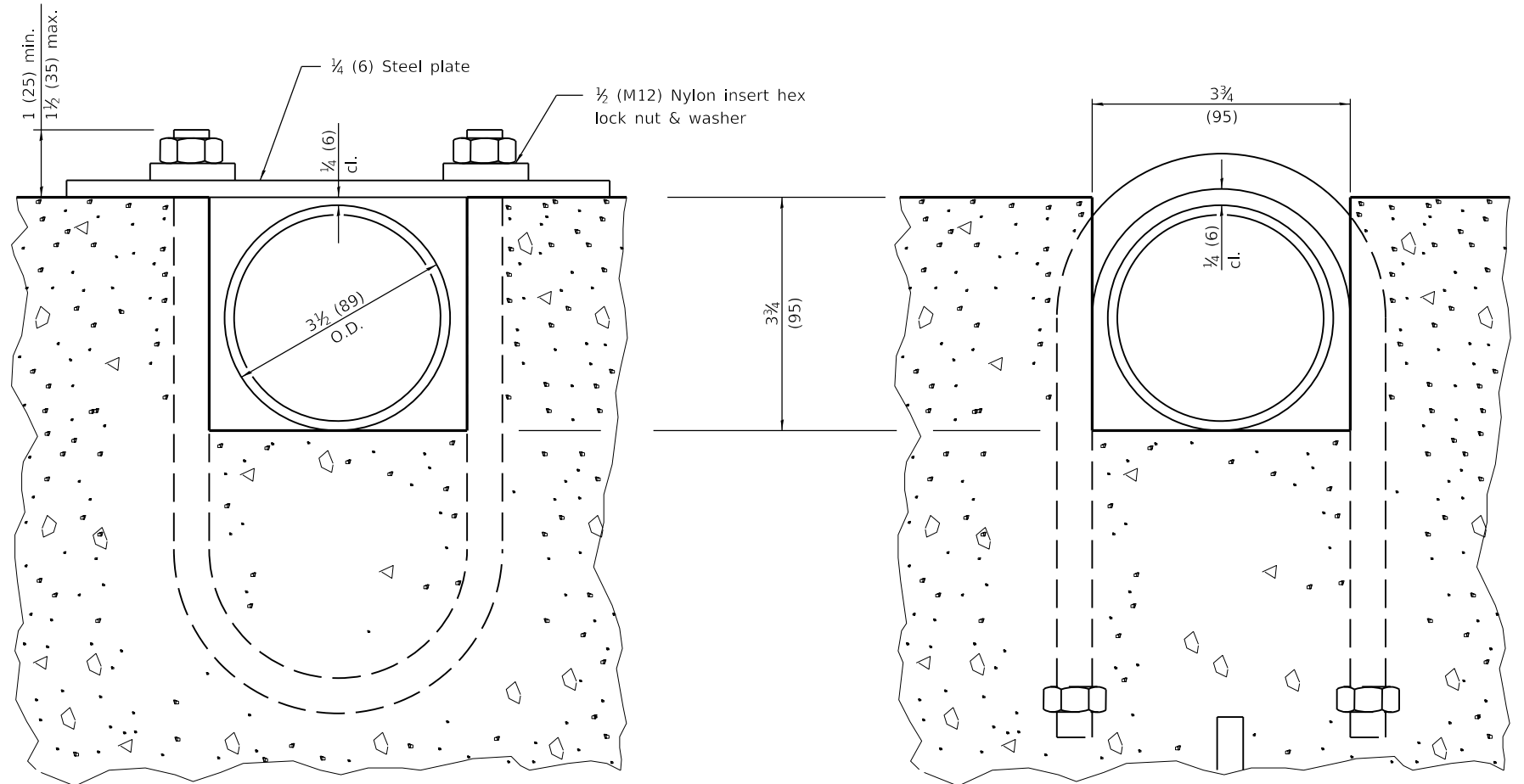
SECTION C-C
