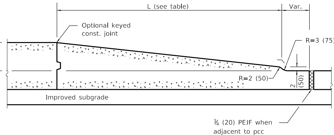
SECTION G-G
