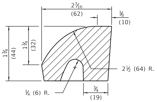
FRONT VANE DETAIL
