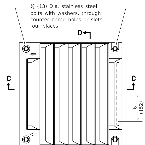
CAST GRATE
