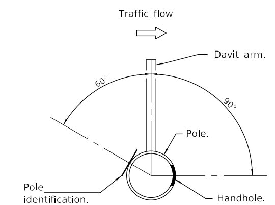
Pole on ground mounted foundation.
