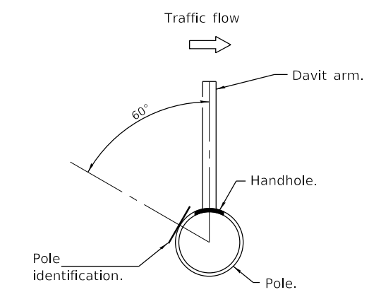
Pole on barrier wall, retaining wall or parapet.
