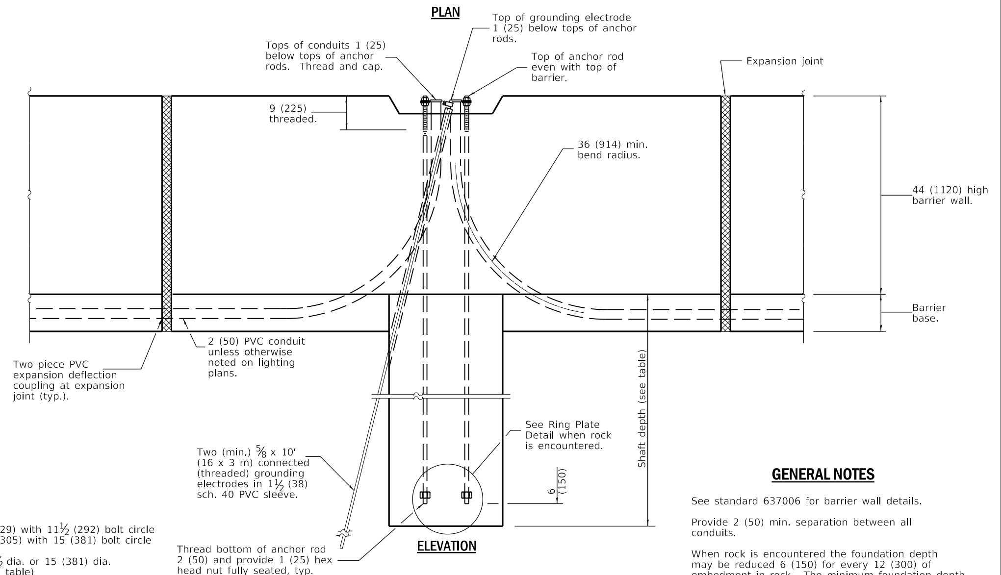
LIGHT POLE FOUNDATION
