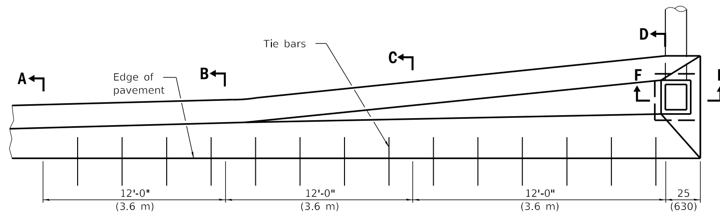
PLAN-DOUBLE OUTLET
