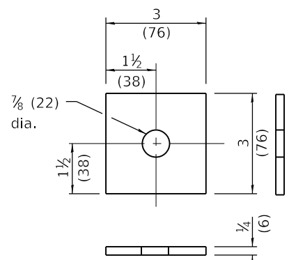
SQUARE WASHER B
