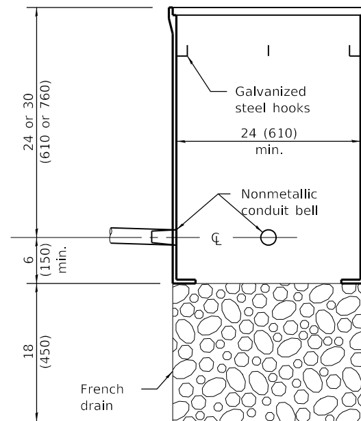
ELEVATION COMPOSITE CONCRETE
