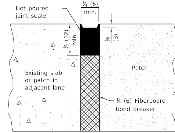
CENTERLINE JOINT
