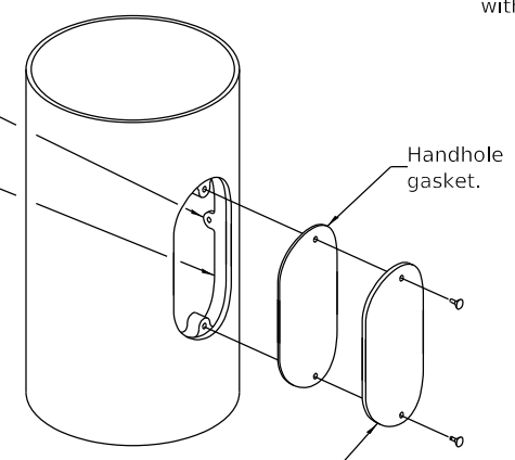
HANDHOLE DETAIL
