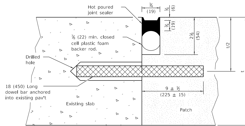
TRANSVERSE JOINT
