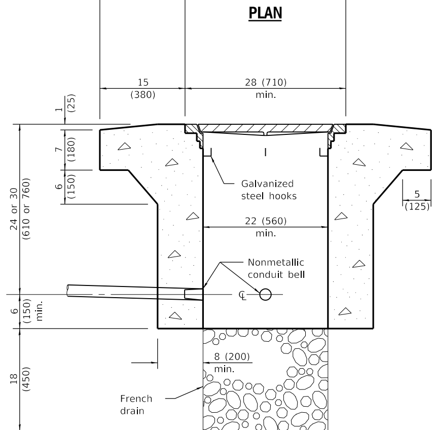
ELEVATION PORTLAND CEMENT CONCRETE HEAVY DUTY
