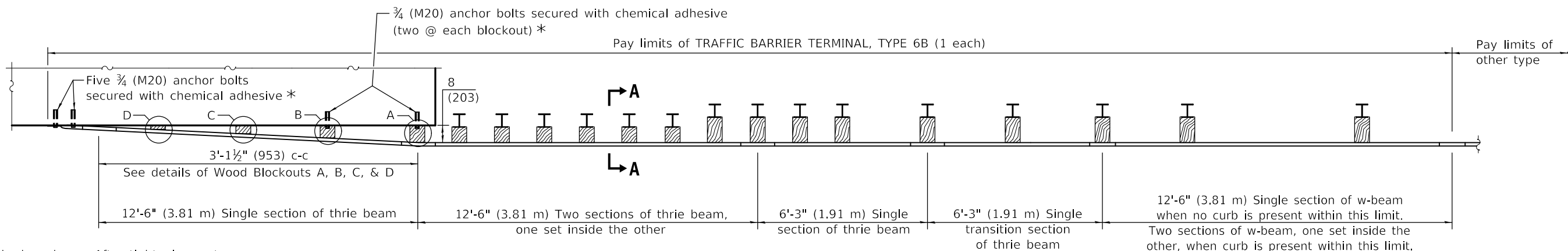
PLAN
