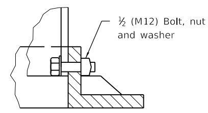
DETAIL OF BOLTING FRAME TO BASE
