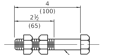
ANCHOR BOLT
