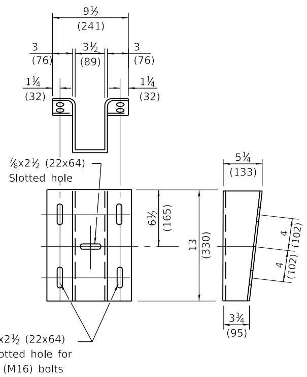
BRACKET U
