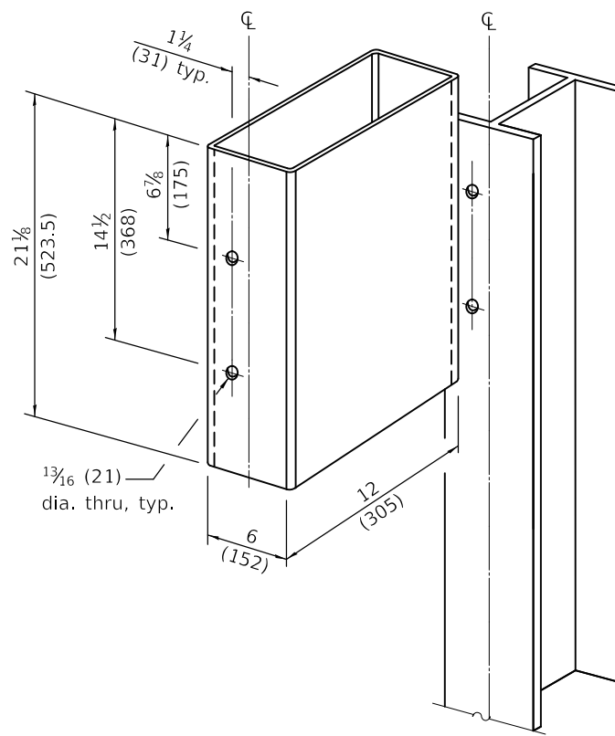
LONG TUBING BLOCKOUT DETAIL
