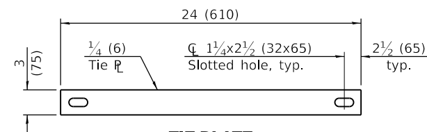
TIE PLATE
