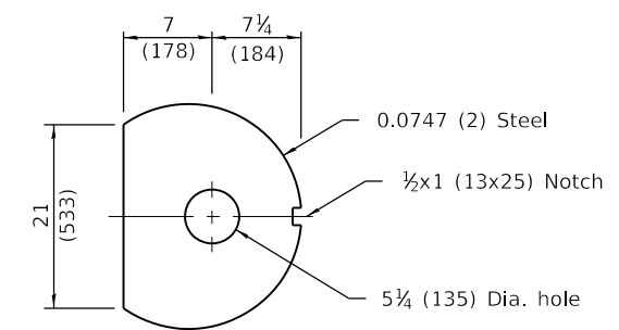
DIAPHRAGM (2 ea.)
