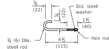
HOOK BOLT G
