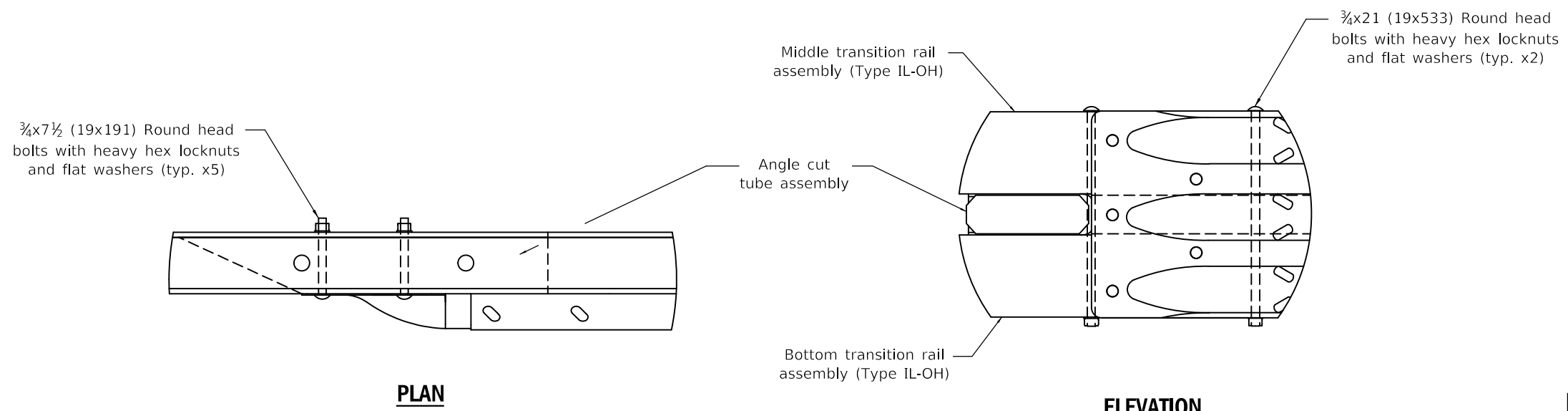
BRIDGE RAIL CONNECTION DETAIL
