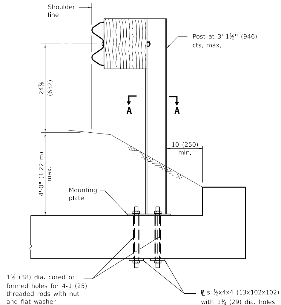
CROSS SECTION
