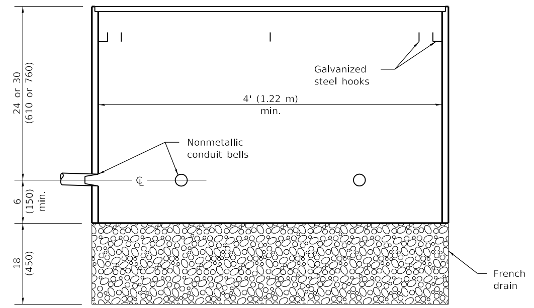
ELEVATION COMPOSITE CONCRETE
