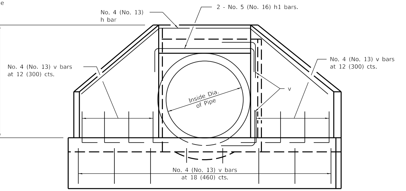
END VIEW
