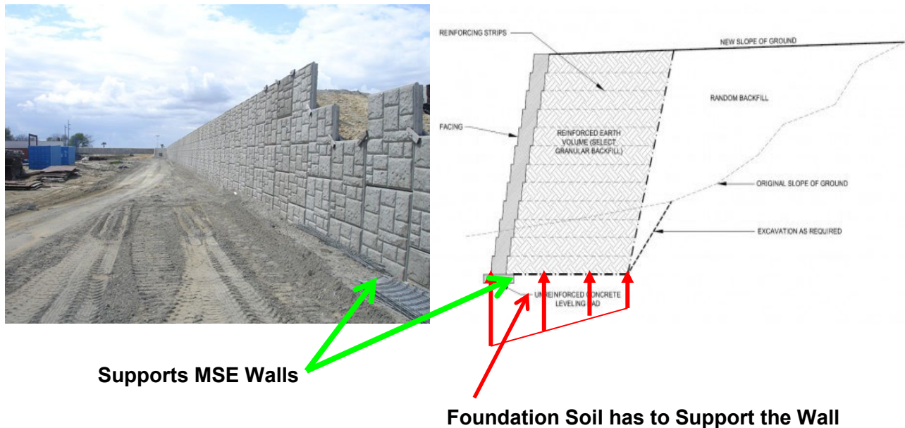
(a) (b) Figure 29. Photo of typical Mechanically Stabilized Earth (MSE) wall (a) with extent of the shallow foundation illustrated (b).
