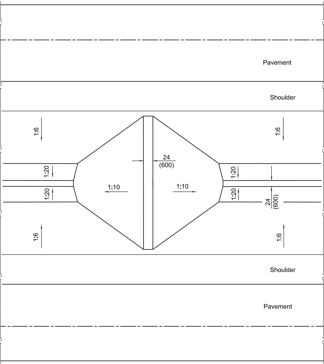
DITCH CHECK FOR WIDE MEDIAN
