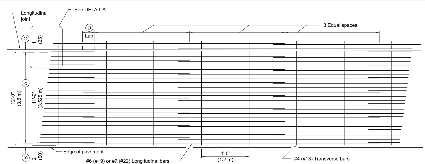
LAP DETAIL I
