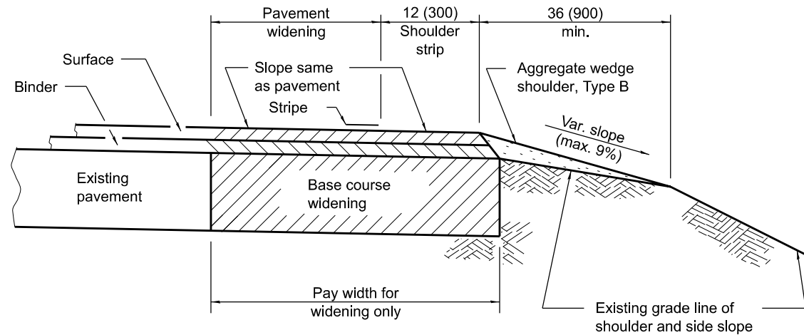
HMA SHOULDER STRIP AND AGGREGATE WEDGE WITH WIDENING (Cross-section A)
