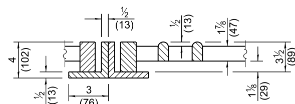
DETAIL C
