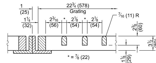
DETAIL B
