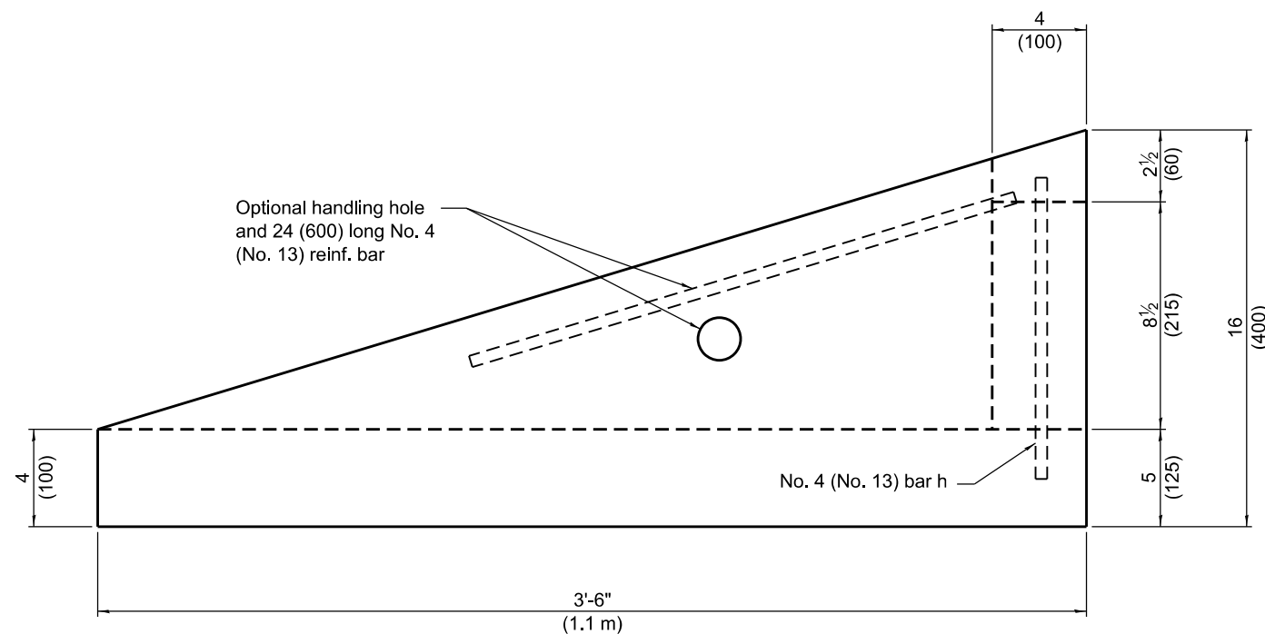
SIDE VIEW
