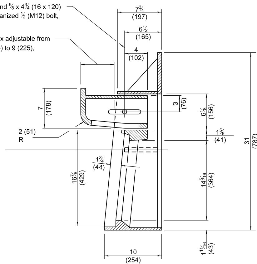
SECTION B-B
