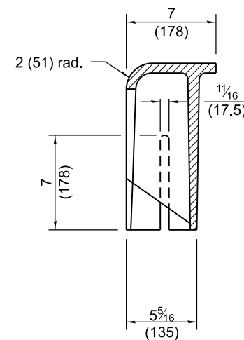
SECTION E-E
