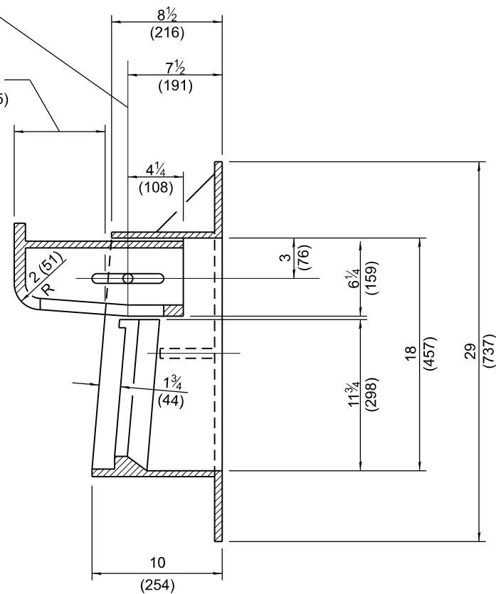
SECTION B-B
