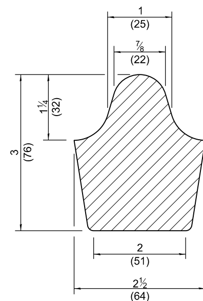
MIDDLE RIB DETAIL
