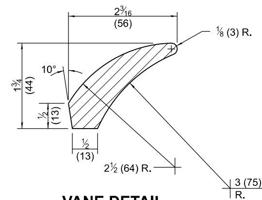
VANE DETAIL
