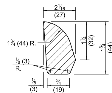
SIDE RIB DETAIL
