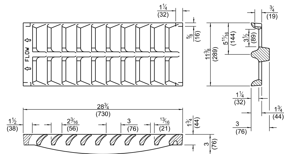
CAST GRATE
