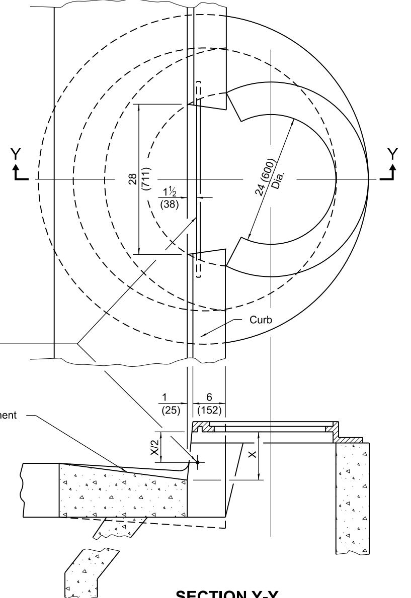
SECTION Y-Y (WITH FRAME)
