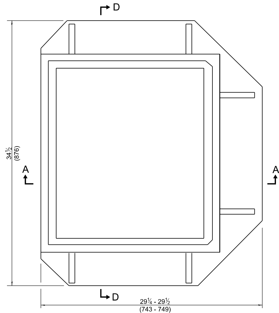
PLAN - FRAME
