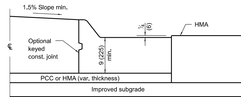
HALF SECTION FOR FLEXIBLE PAVEMENT
