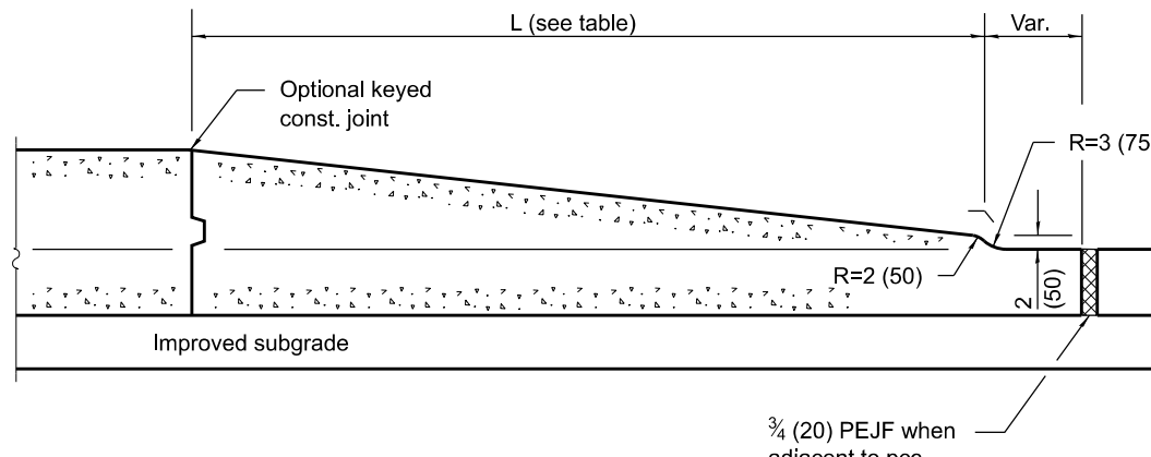
SECTION G-G
