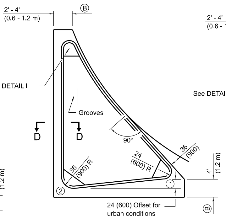
INTERMEDIATE ISLAND (FOR RIGHT TURN LANE DESIGN)
