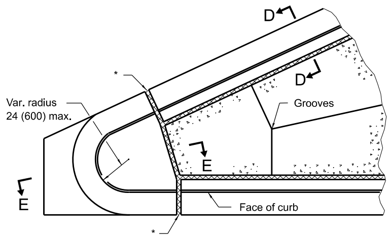
DETAIL I
