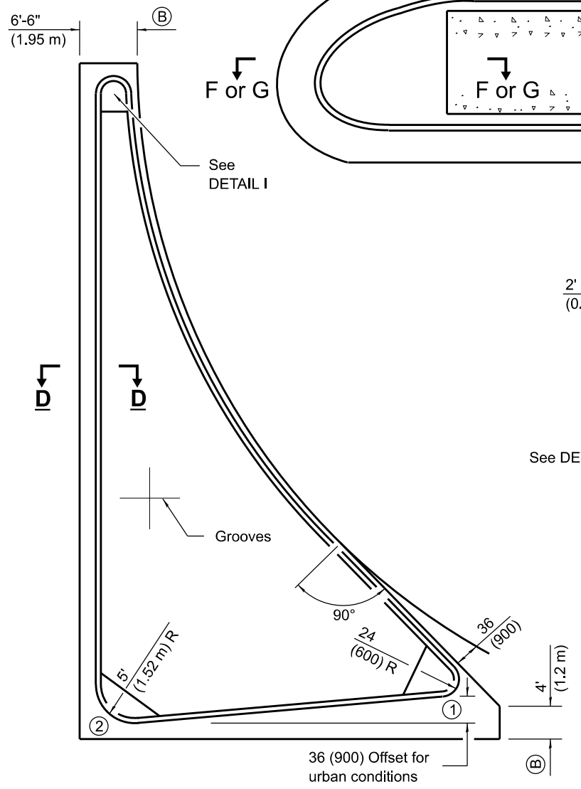
LARGE ISLAND (FREE FLOW DESIGN)
