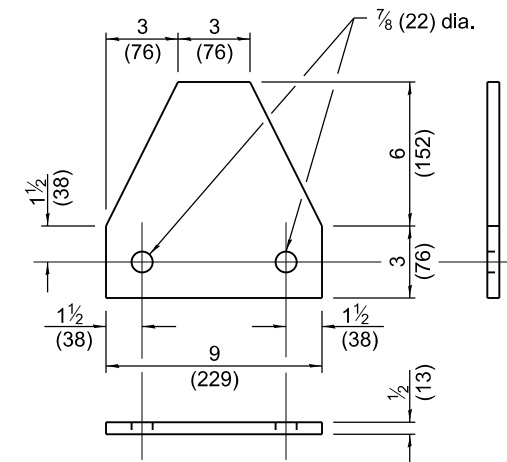
PLATE E
