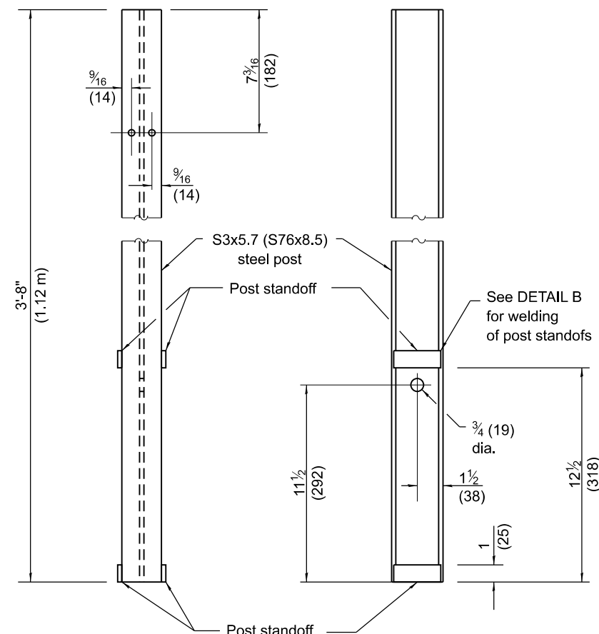
STEEL POST
