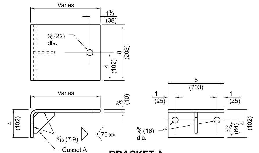
BRACKET A
