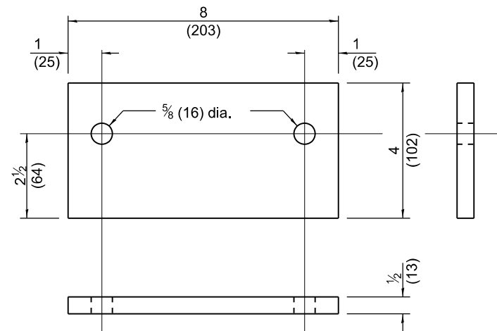
PLATE C
