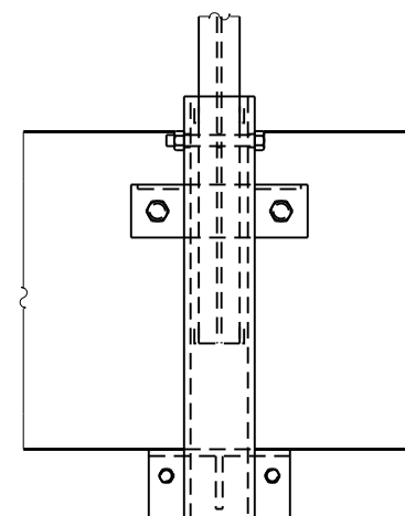
CASE II, (H+T-R) < 18 (457), SIDE-MOUNT THROUGH-BOLT
