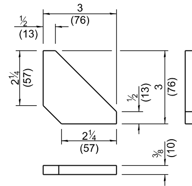
GUSSET A
