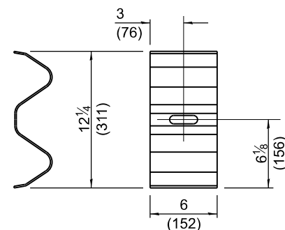
BACKUP PLATE
