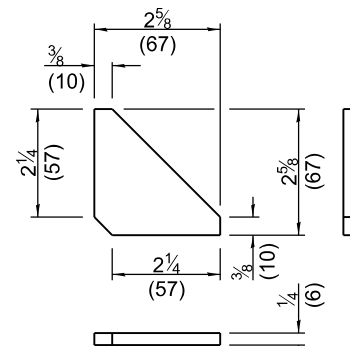
GUSSET C
