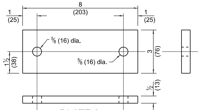
PLATE A
