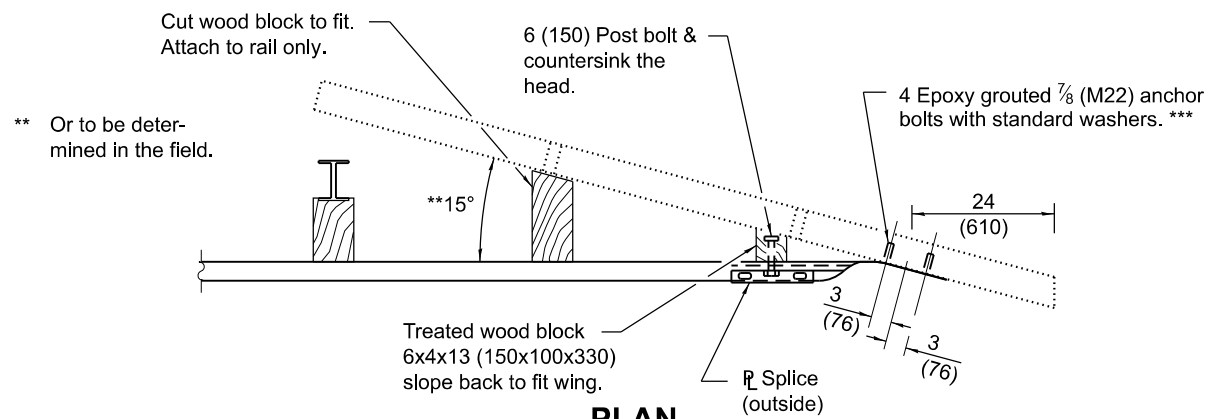
PLAN FLARED WING
