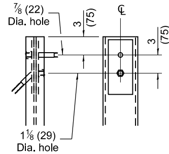
DETAIL M
