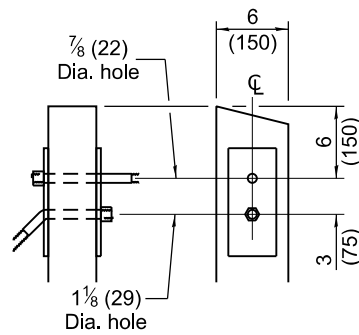
DETAIL H
