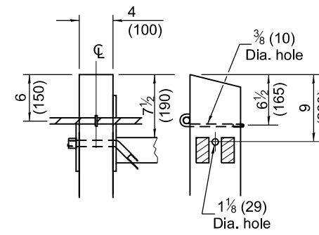
DETAIL K
