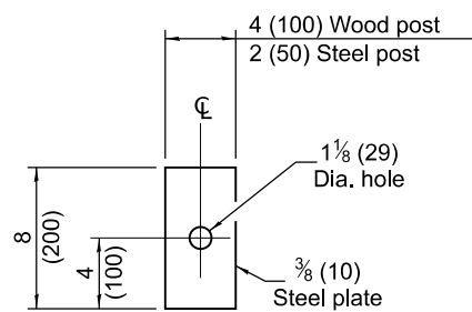
PLATE C
