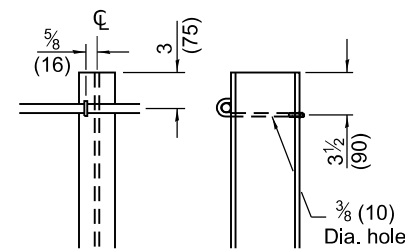
DETAIL J
