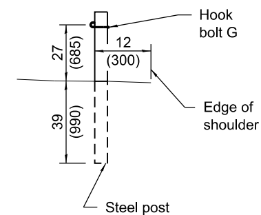
VIEW Y-Y
