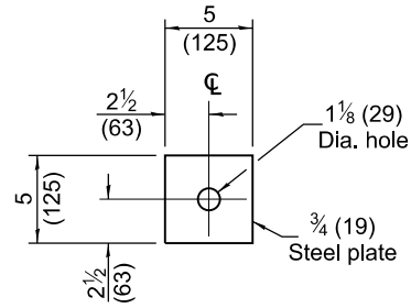
PLATE B
