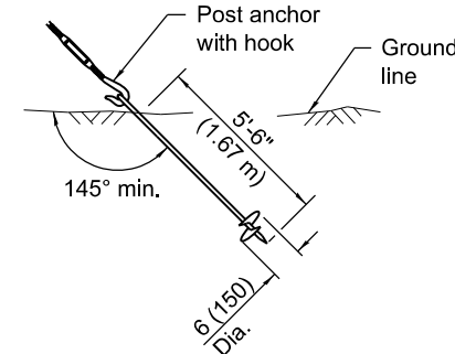
STEEL SCREW
