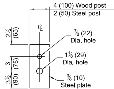
PLATE E
