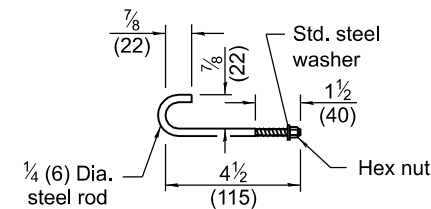
HOOK BOLT G
