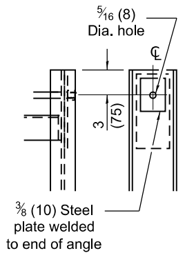
DETAIL R
