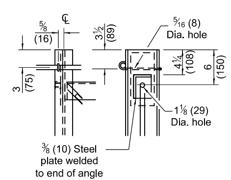
DETAIL P
