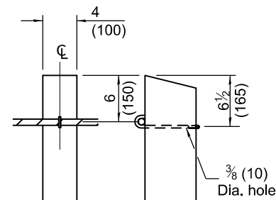
DETAIL J
