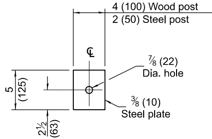
PLATE D
