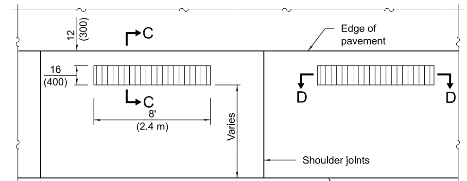
PLAN (Formed Alternate for PCC Shoulders) Center rumblestrips between the shoulder joints.
