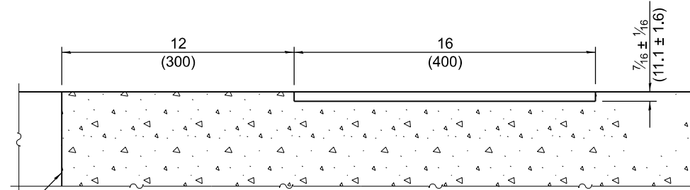
SECTION B-B
