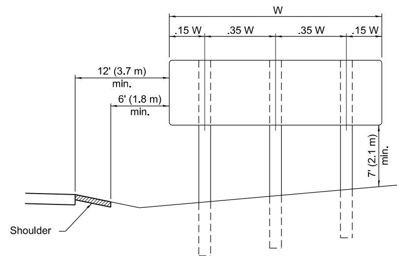
POST SPACING FOR NON-FREEWAY SIGN PANELS
