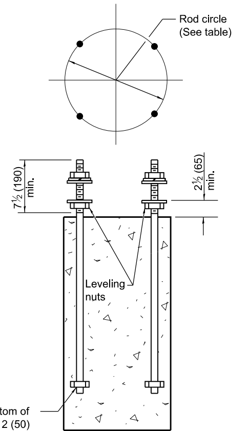
ANCHOR ROD DETAIL
