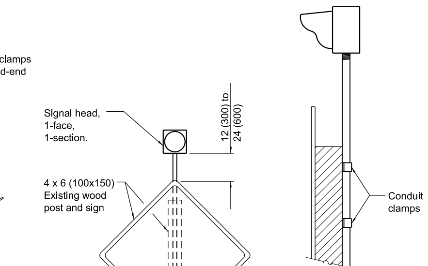
MOUNTING DETAIL
