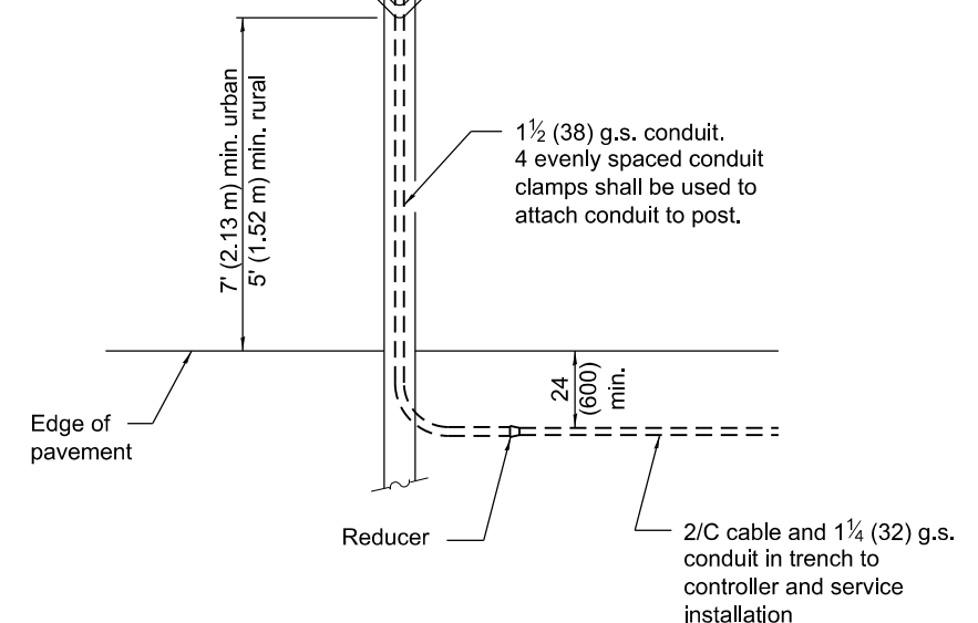
POST MOUNTED FLASHING BEACON
