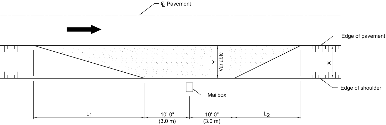
TYPICAL APPLICATION
