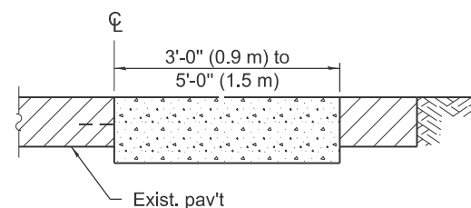
SECTION F-F
