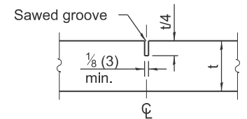
DETAIL OF SAWED CONTRACTION JOINT
